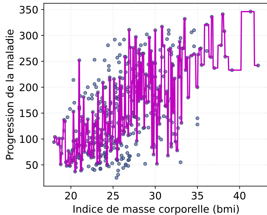
(a) k = 1
