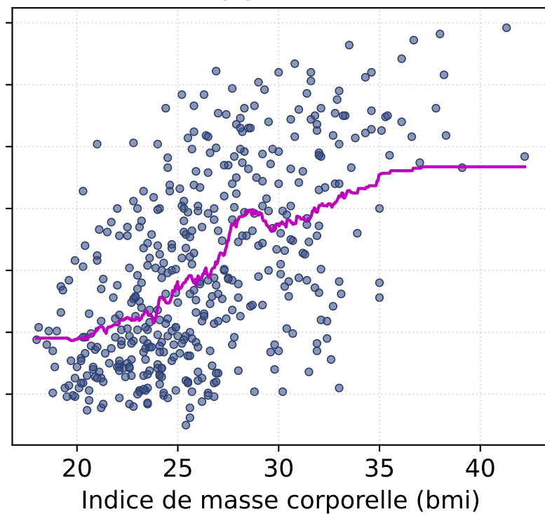
(c) k = 50
