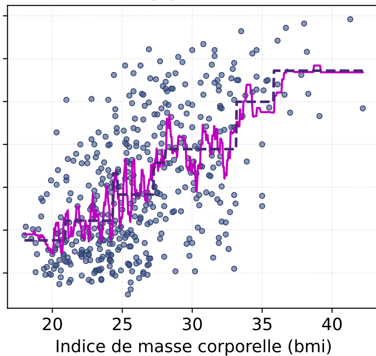
(b) k = 10
